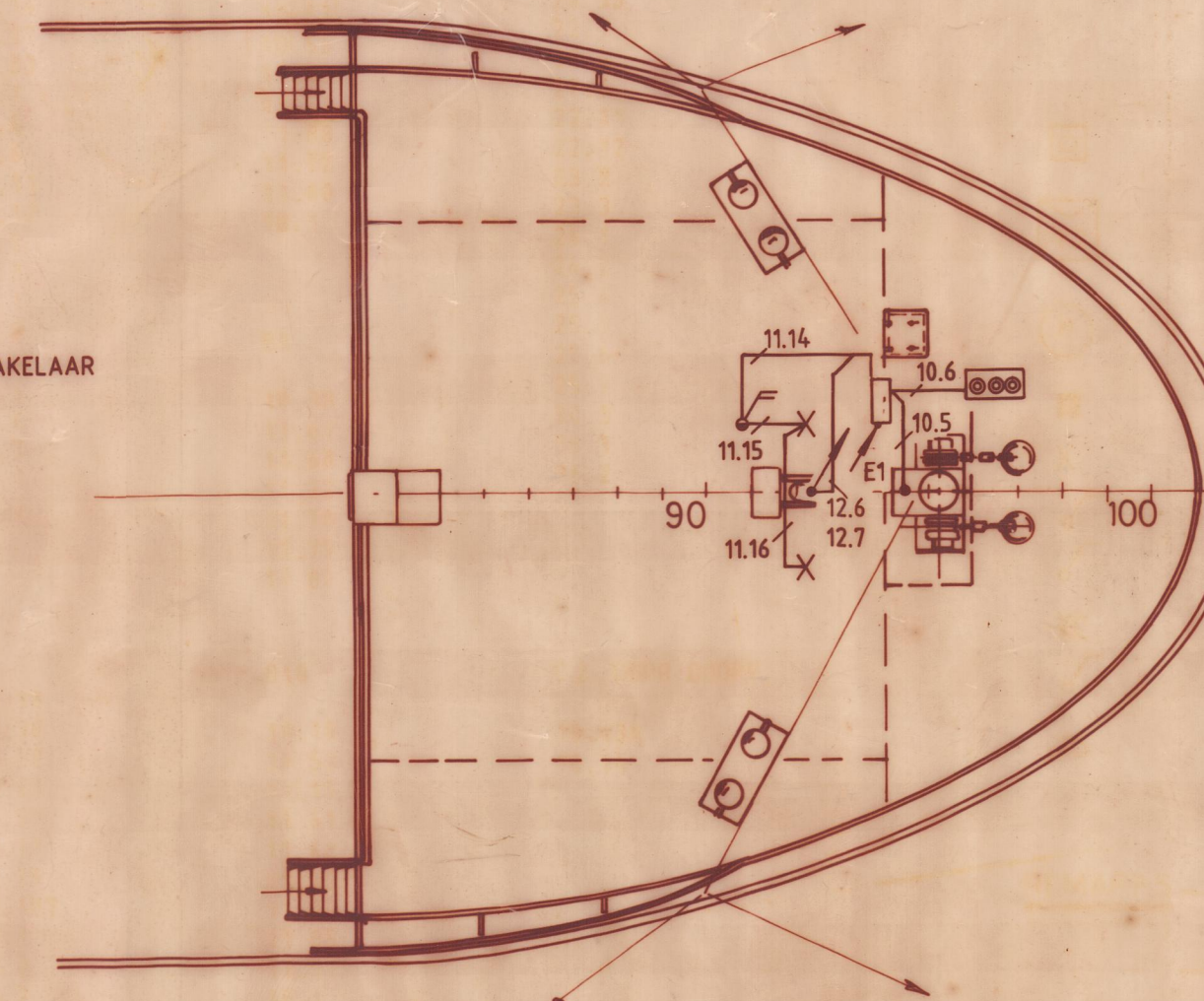
Forecastledeck
