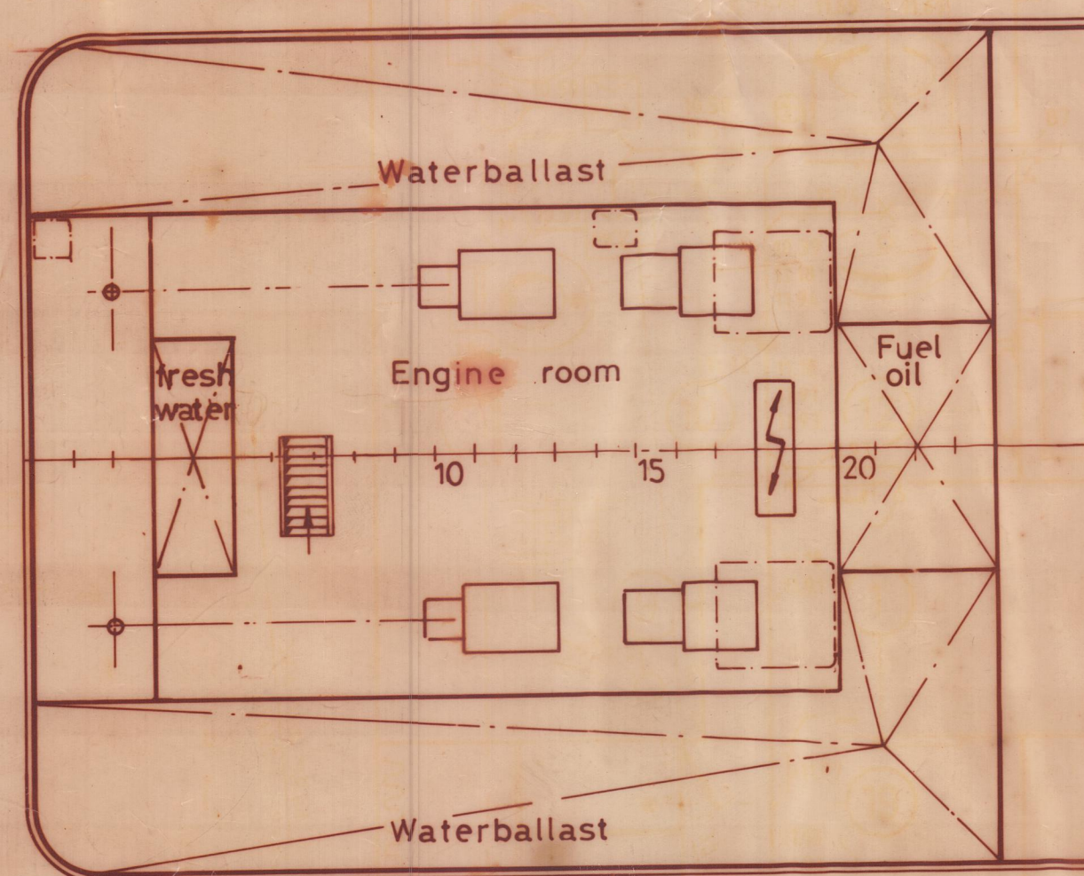
Section below maindeck
